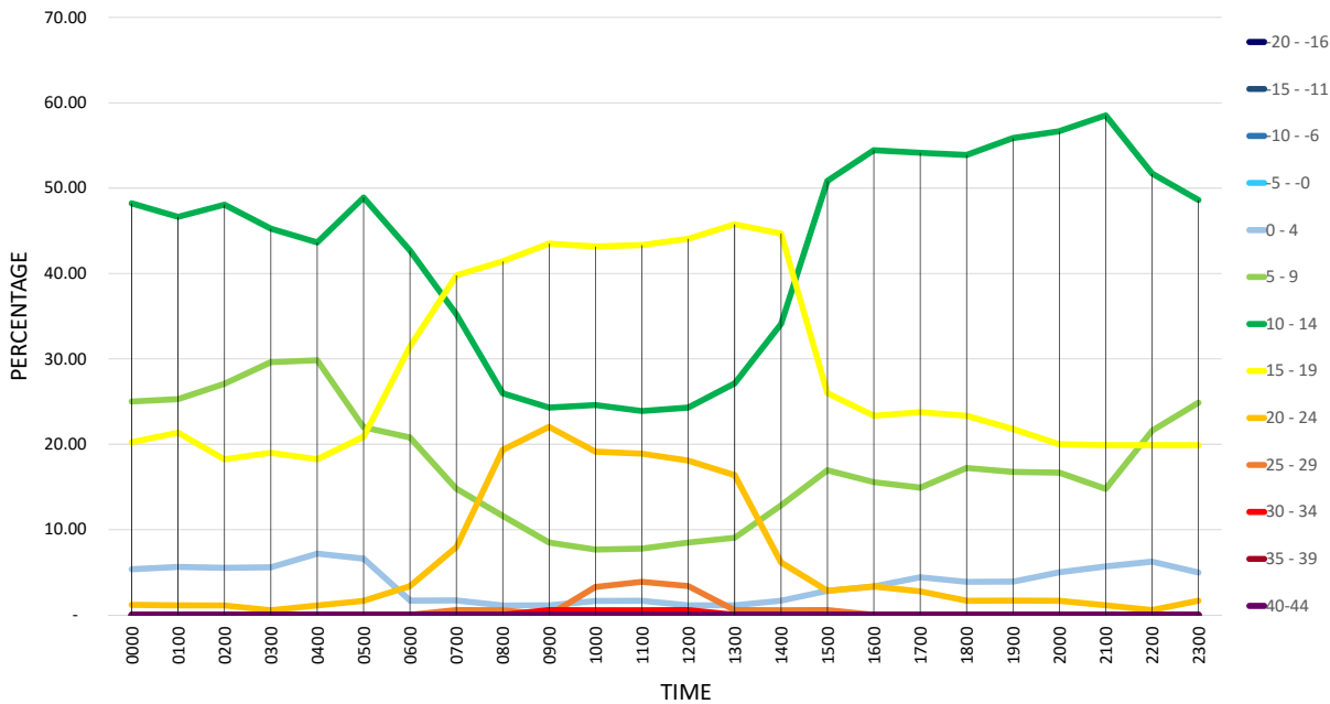
UGSB - Temperature (November 2010-2015)
