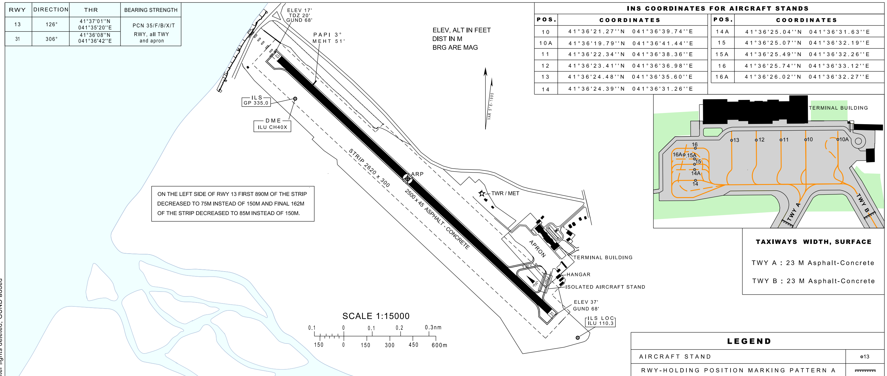
MARKING AIDS RWY 13/31 AND EXIT TWY
